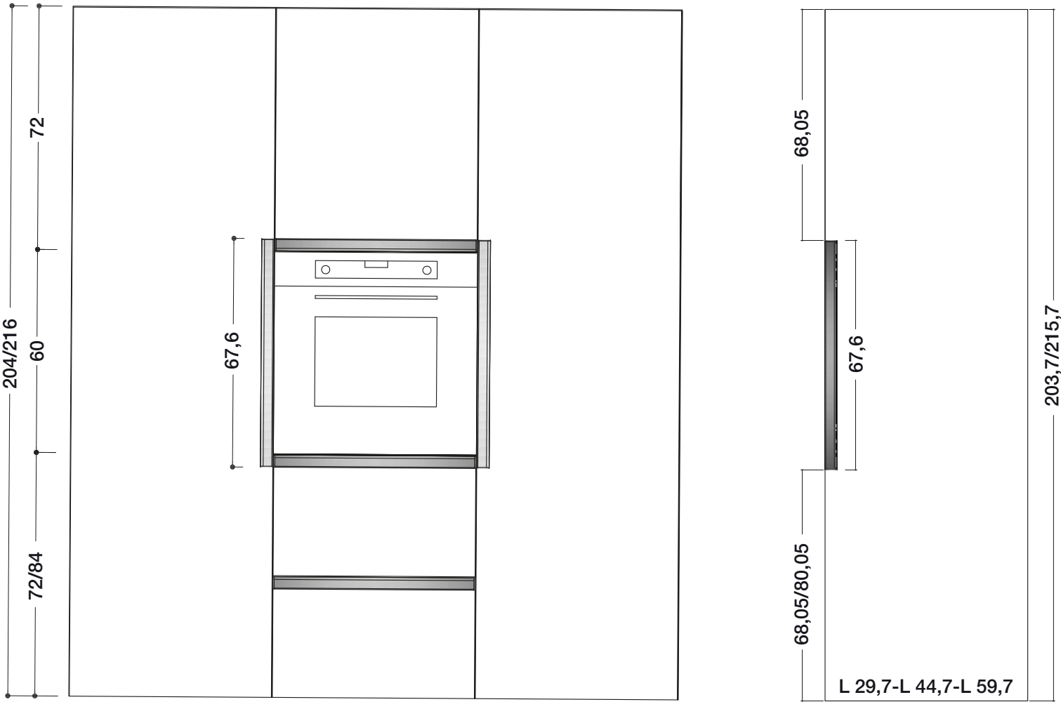
Anta monoporta con maniglia in verticale Single-door with handle vertical
